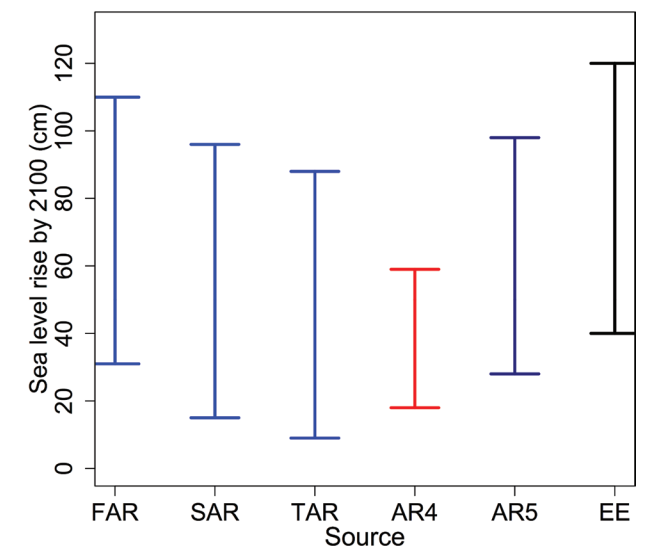
FIG. 2. Reported upper and lower bounds of global sea level rise by ca. 2100 from summary reports in the IPCC assessment reports and a recent expert elicitation analysis: (left to right) First Assessment Report (FAR; increase by 2100; Rick et al. 2011) in 1991, Second Assessment Report (SAR; increase by 2100 relative to 1990; Rick et al. 2013) in 1996, Third Assessment Report (TAR; increase by 2100 relative to 1990; Houghton et al. 2001) in 2001, Fourth Assessment Report (AR4; 5%–95% range on increase by 2090–99 relative to 1980–99, with table notation “excluding future rapid dynamical changes in ice flow”; Alley et al. 2007) in 2007, Fifth Assessment Report (AR5; 17%–83% range on increase by 2100 relative to 1985–2005; Alexander et al. 2013) in 2013, and an expert elicitation analysis (EE; 17%–83% range on increase by 2100 relative to 2000; Horton et al. 2014).
