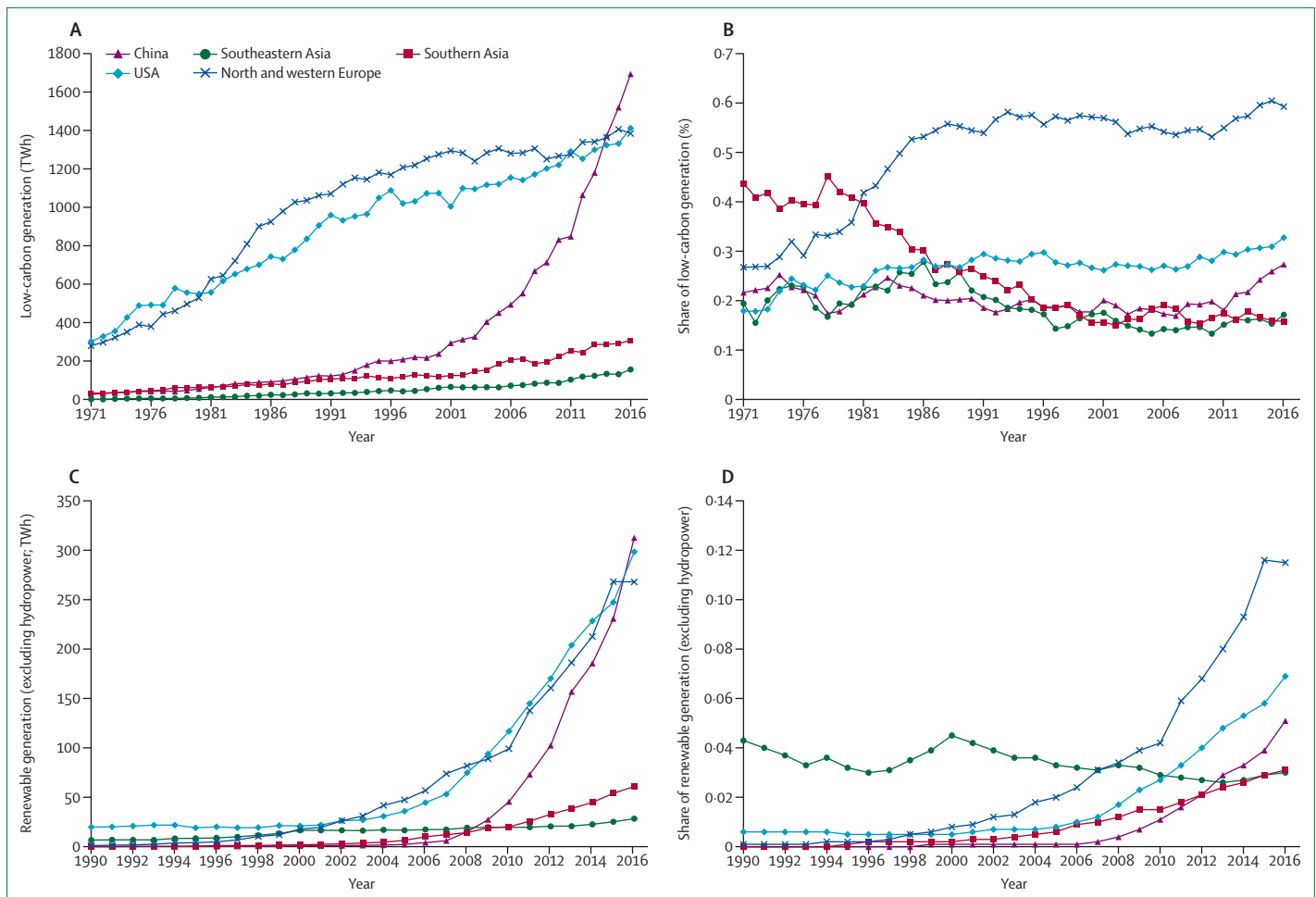
Figure 14: Renewable and low-carbon emission electricity generation
