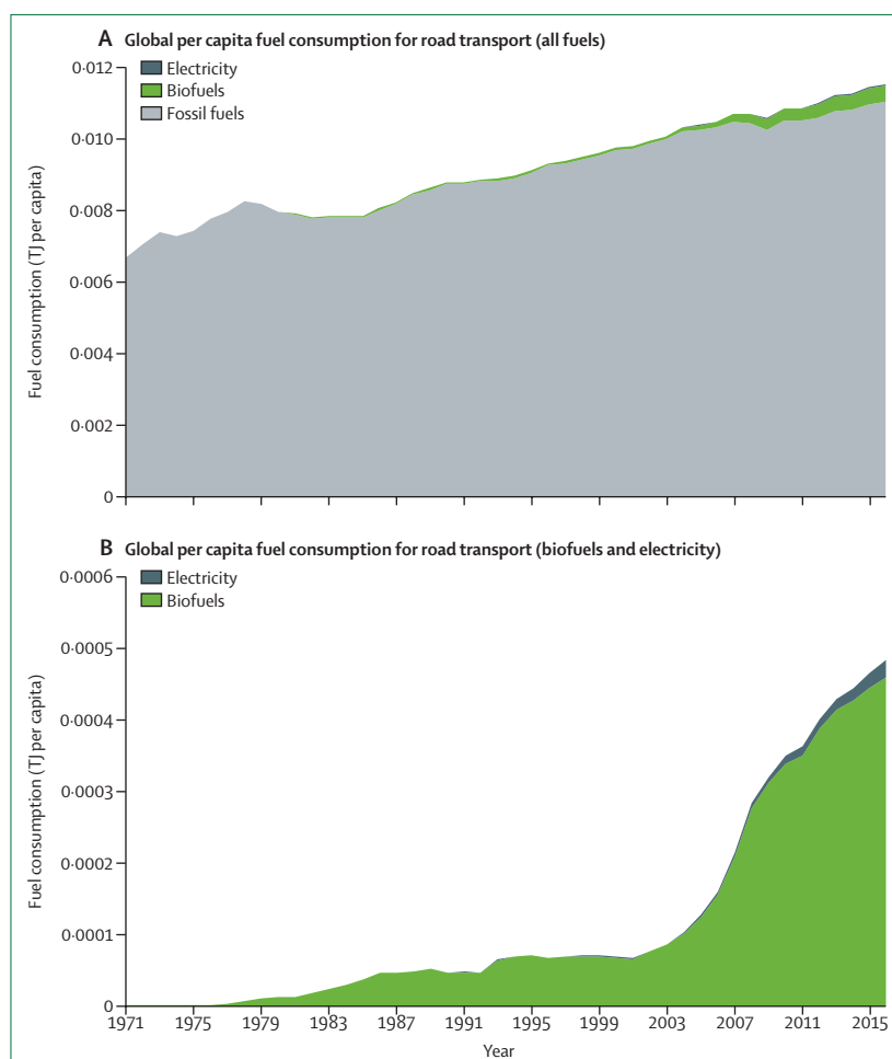
Figure 17: Per-capita fuel use by type (Tj per capita) for road transport
