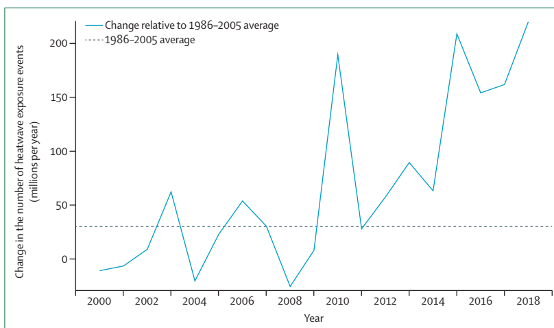
Figure 1: Change in the number of heatwave exposure events in people aged 65 years and older, compared with the historical 1986–2005 average number of events
