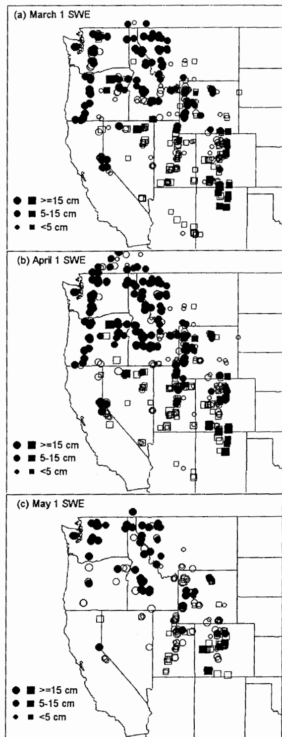
FIG. 4. Locations of snow-course measurement sites used in the analysis of SWE. Trends in accumulated snowpack (cm) for (a) 1 Mar, (b) 1 Apr, and (c) 1 May are shown. Circles indicate decreasing SWE values, and squares indicate increasing SWE values; filled (open) symbols represent stations passing (failing) two-tailed t tests of significance.
