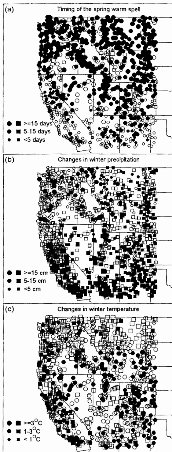
FIG. 6. Locations of weather stations used in the analysis of climate variations. (a) Changes in the timing of the spring warm spell (day); (b) changes in winter precipitation (cm); and (c) changes in winter temperature ( ^{\circ}\text{C} ). Coding is the same as in Fig. 4.
