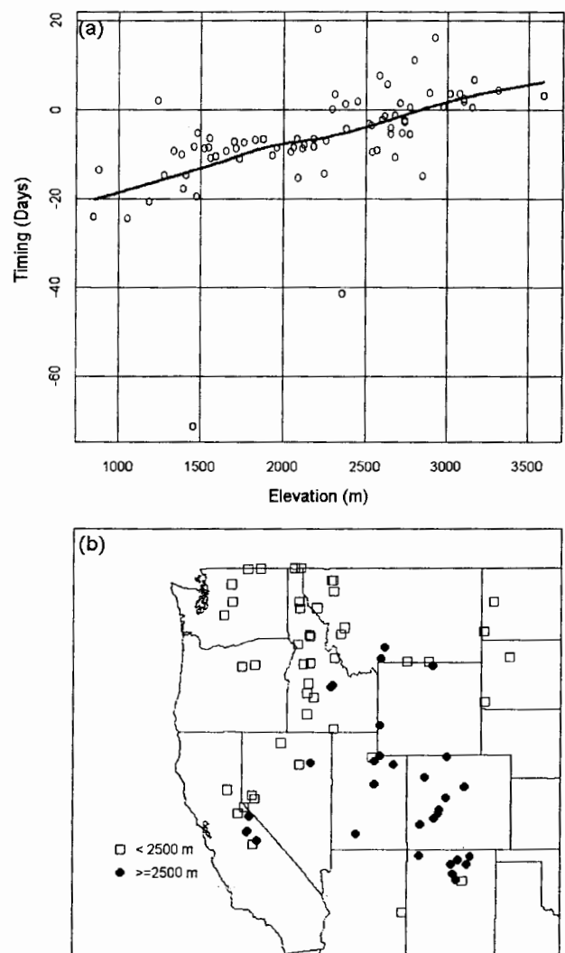
FIG. 3. (a) Scatterplot comparing the trends in the timing of 50% of annual streamflow against the mean basin elevations, and (b) a map illustrating spatial distribution of basins where the mean basin elevation (m) is above 2500 m. Note that mean basin elevations are considerably higher in the interior west.
