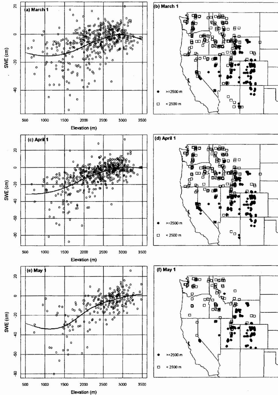
FIG. 5. Scatterplots comparing the trends in SWE (cm) against snow-course elevation (m) for measurements taken on (a) 1 Mar, (c) 1 Apr, and (e) 1 May, and (b), (d), (f) maps illustrating the spatial distribution of stations where the elevation is above/below 2500 m. Station locations are more or less preserved in each month, but the number of stations used in the analysis varies for each month.
