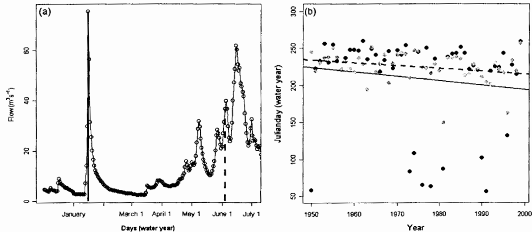
FIG. 1. (a) Daily hydrograph for water year 1974 of the American River near Nile, WA (USGS gauge 12488500). Solid line indicates the data of the annual maximum flow; this peak is likely the result of rainfall. Dashed line indicates the day corresponding to 50% of the annual flow; this date precedes the main snowmelt peak by about 10 days but coincides relatively closely to the centroid of the snowmelt hydrograph. (b) Trends in the timing (day of the water year) of peak flows on the American River for the period 1950–99. Black circles indicate dates corresponding to the annual maximum flow; a number of these flows were produced by rainfall rather than snowmelt. Gray circles indicate dates corresponding to 50% of the annual flow; nearly all of these dates fall within the period of snowmelt streamflow. The trend formed from annual peaks (solid line) is not statistically significant, whereas the trend formed by selecting peaks in snowmelt (dashed line) is significant at the 0.10 level.
