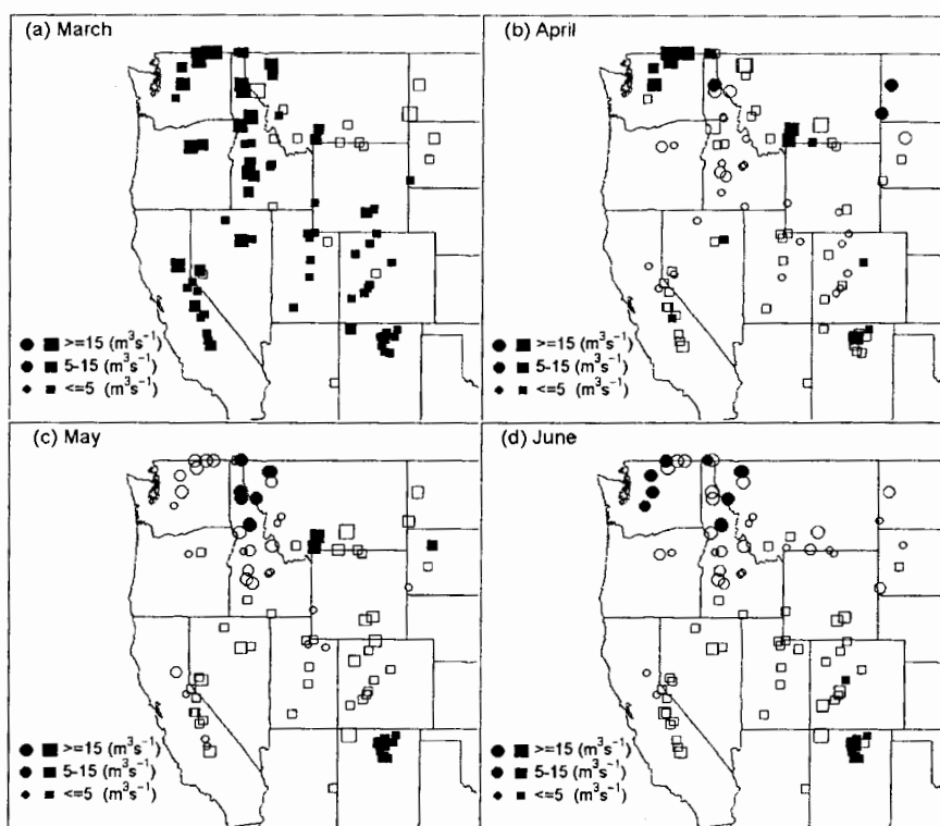
FIG. 9. Trends in monthly streamflow ( \text{m}^3 \text{s}^{-1} ) for (a) Mar, (b) Apr, (c) May, and (d) Jun. Coding is the same as in previous figures.
