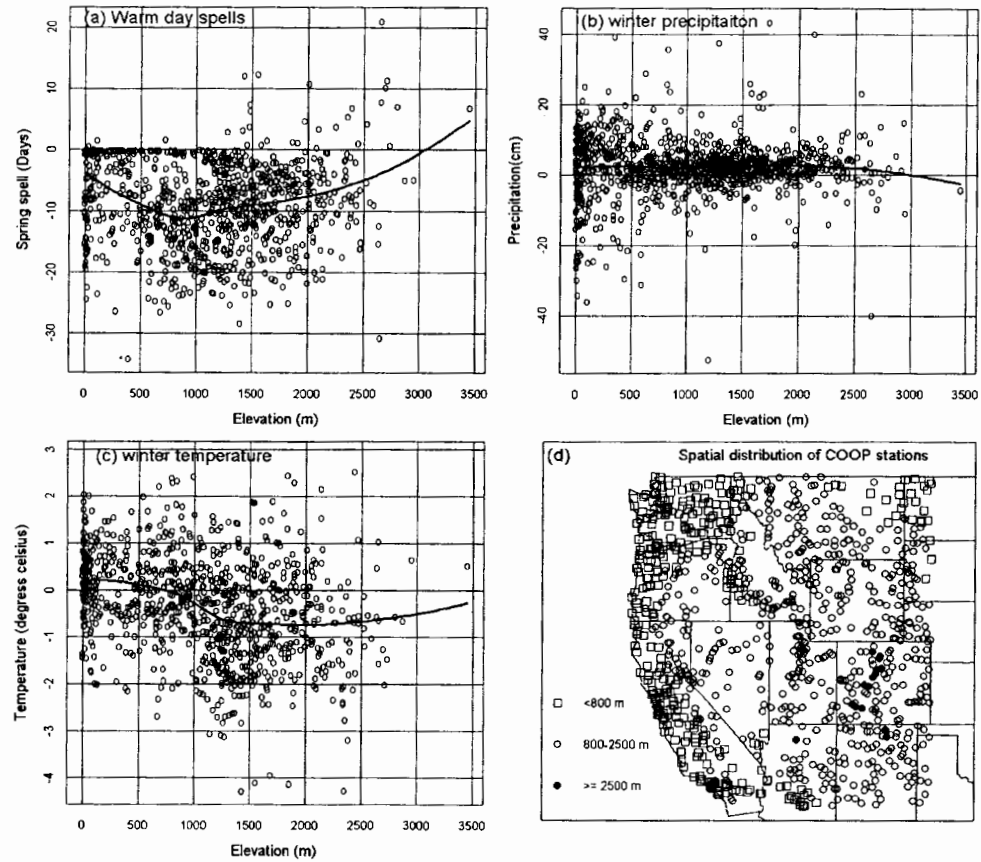
FIG. 7. Scatterplots showing relations between weather station elevation and trends in (a) warm-day spells, (b) winter precipitation, and (c) winter temperature; and (d) a map illustrating the spatial distribution of COOP stations below 800 m (squares), between 800 and 2500 m (open circles), and above 2500 m (filled circles). Note that there are very few COOP stations at high elevations.
