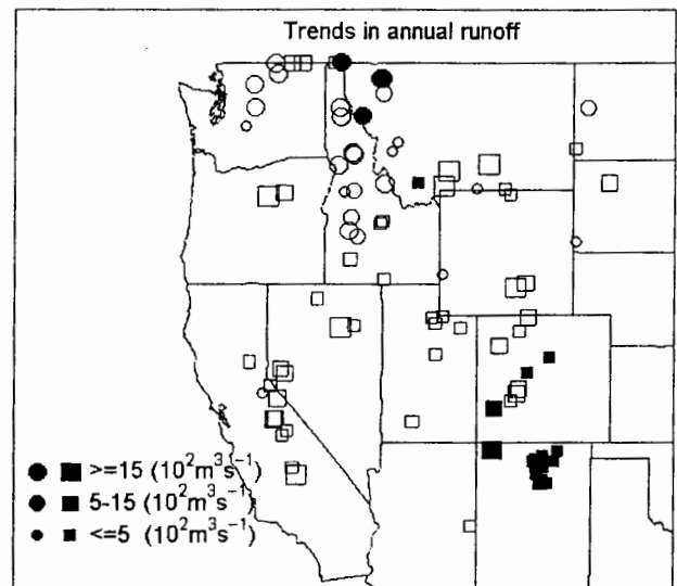
FIG. 8. Trends in annual streamflow ( 100 \text{ m}^3 \text{ s}^{-1} ) at USGS gauging stations. Coding is the same as in previous figures.
