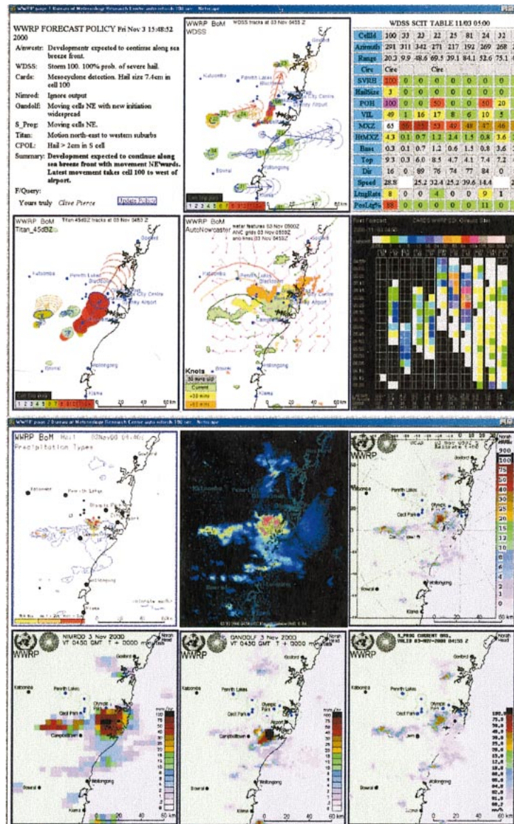
FIG. 1. Example of WWRP S2000 FDP forecaster Web-based guidance products. (a) WWRP summary panel and severe weather guidance that comprises six panels. (top row) System status and WWRP guidance summary with capability for forecaster query, followed by a schematic representation of storm tracks and forecasts color coded by intensity and, in tabular form a cell information summary indicating the presence of severe weather. The next row shows (left to right) major cell tracks and forecasts, derived surface winds with major storm cells and convergent boundaries indicated, and point forecasts of rainfall. (b) WWRP FDP precipitation forecast products. (top row) Polarimetric radar-derived rain-rate analysis with superimposed hail sizes; a standard BoM radar reflectivity and (bottom row) quantitative rainfall forecasts from different FDP systems.
