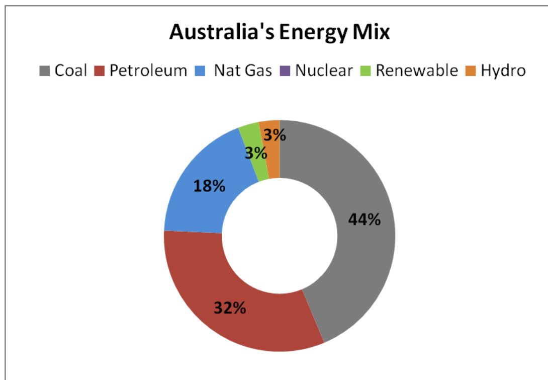
Figure 4. Australia's 2004 energy mix showing the consumption of 5.3 quadrillion BTUs. There was no nuclear power in Australia in 2004.
