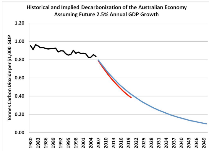
Figure 3. Past rates of decarbonization of the Australian economy, 1980-2006, and implied rates of decarbonization assuming 2.5% annual GDP growth for the 2020 (25% reduction target in red) and 2050 targets (60% reduction target in blue).
