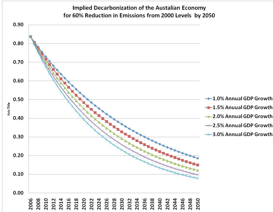
Figure 1. Implied rates of decarbonization of the Australian economy for various rates of GDP growth, 2007 to 2050.
